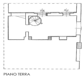
PIANO TERRA
